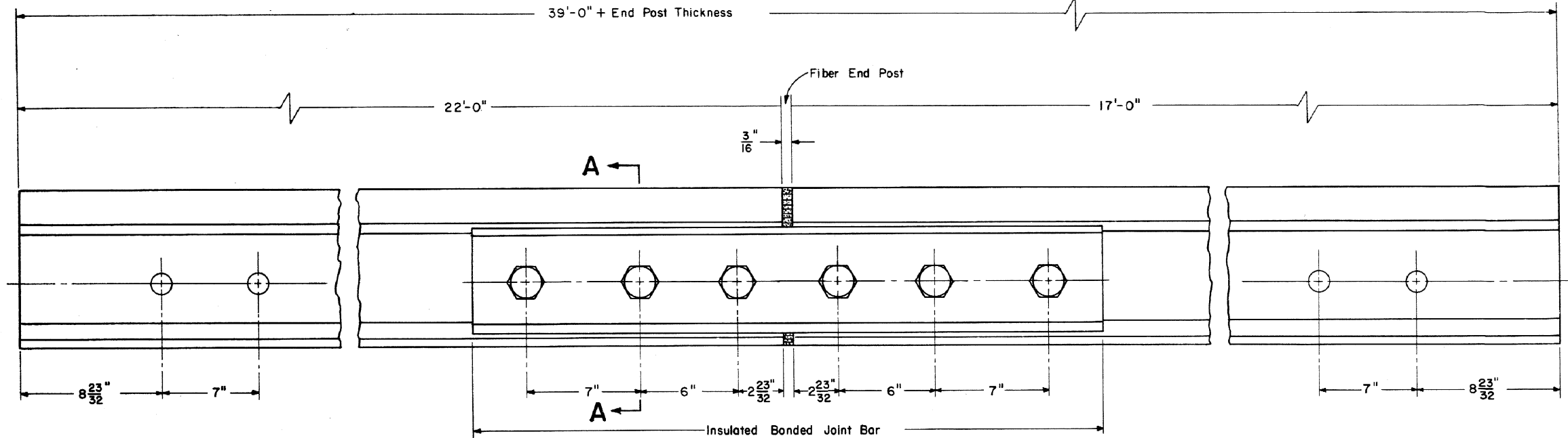
SIDE VIEW
