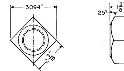
SQUARE NUT
