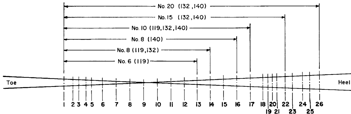
BOLT LOCATIONS
