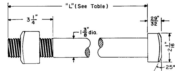
FROG BOLT
