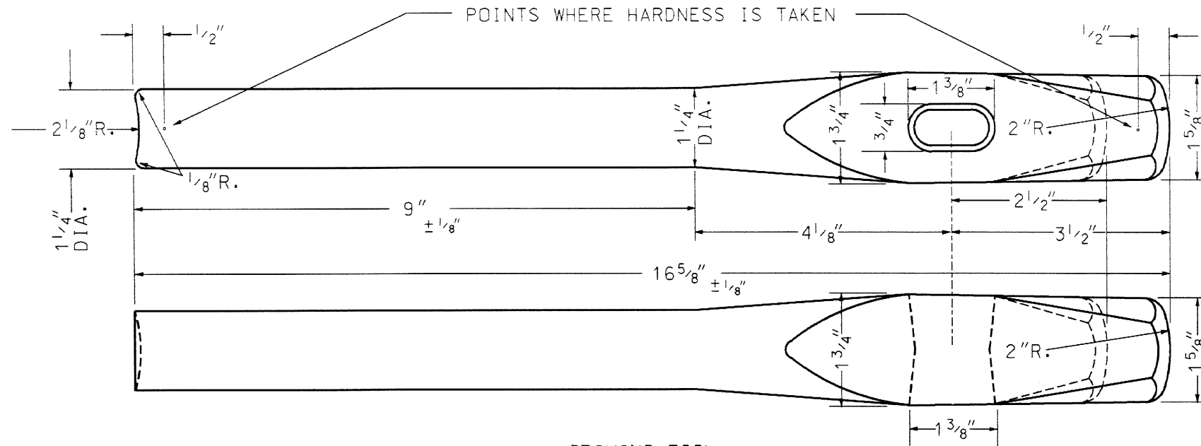
SPIKING TOOL AREA PLAN 41-94 ITEM NUMBER 45-739404
