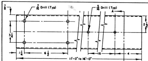
BASE SECTION Fiber Reinforced Polyglass
