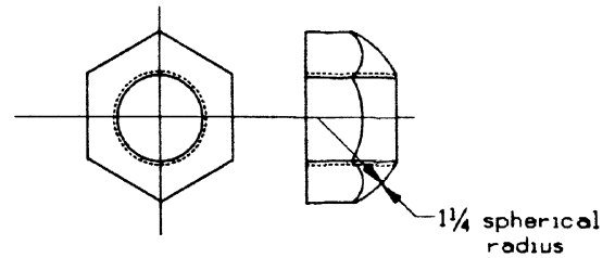
1/4 - 7 NC 2 hvy semi-finished hex nut except as shown
